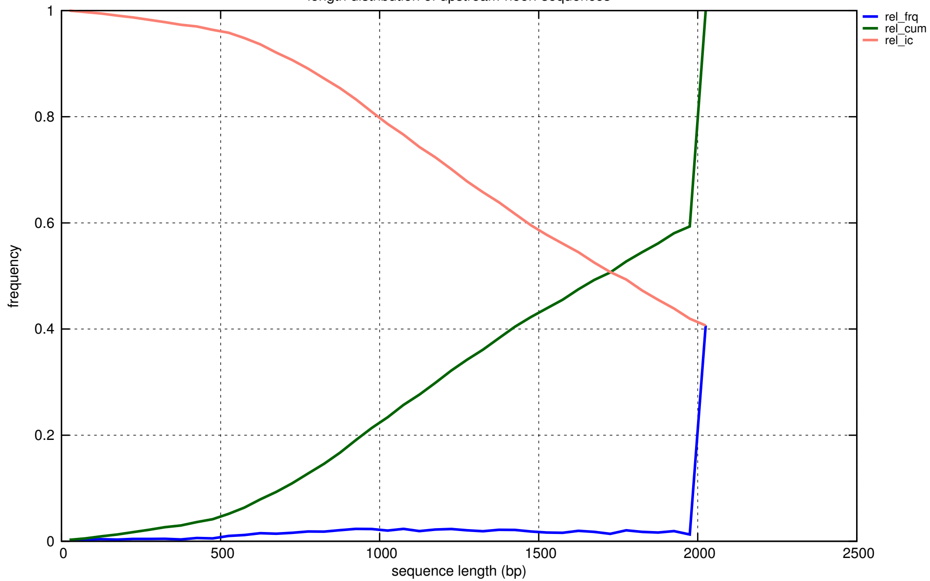
Plasmodium falciparum length distribution of upstream-noorf sequences
